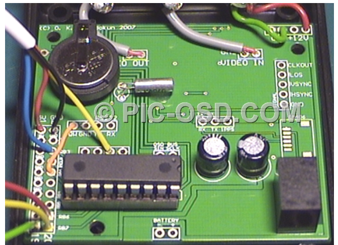
The board with connections made
