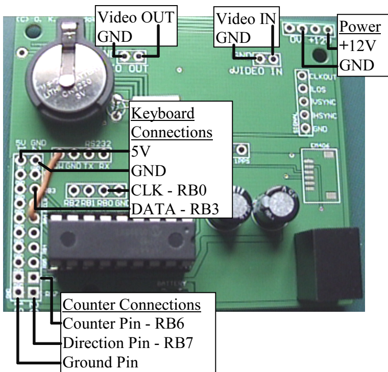
Keyboard and counter connection points on the board
